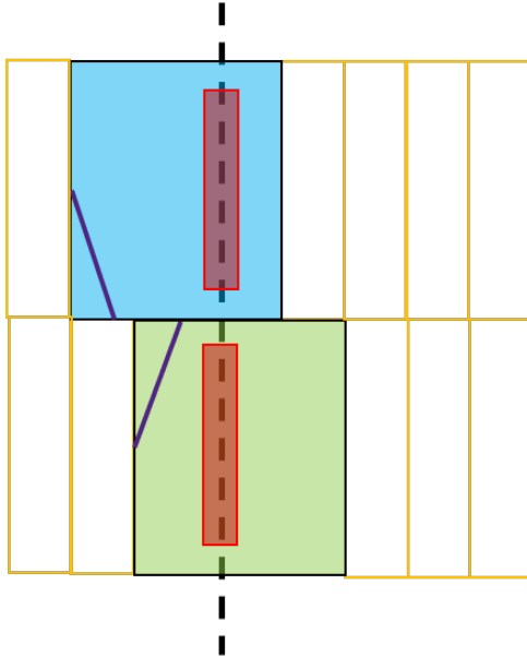
Figure 19 Equivalent Cells With Different Pin Locations
