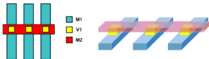
Figure 70 Single-Level Pattern-Based Must-Join Pin Connection
