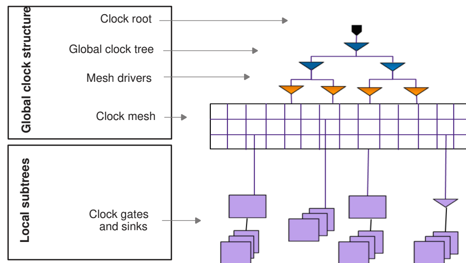
Figure 46 Structural Multisource Clock Tree
