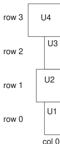
Figure 136 Bottom-Right-Aligned Relative Placement Group
