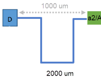
Figure 116 Minimum Wire Length Constraint for the a2/A Pin
