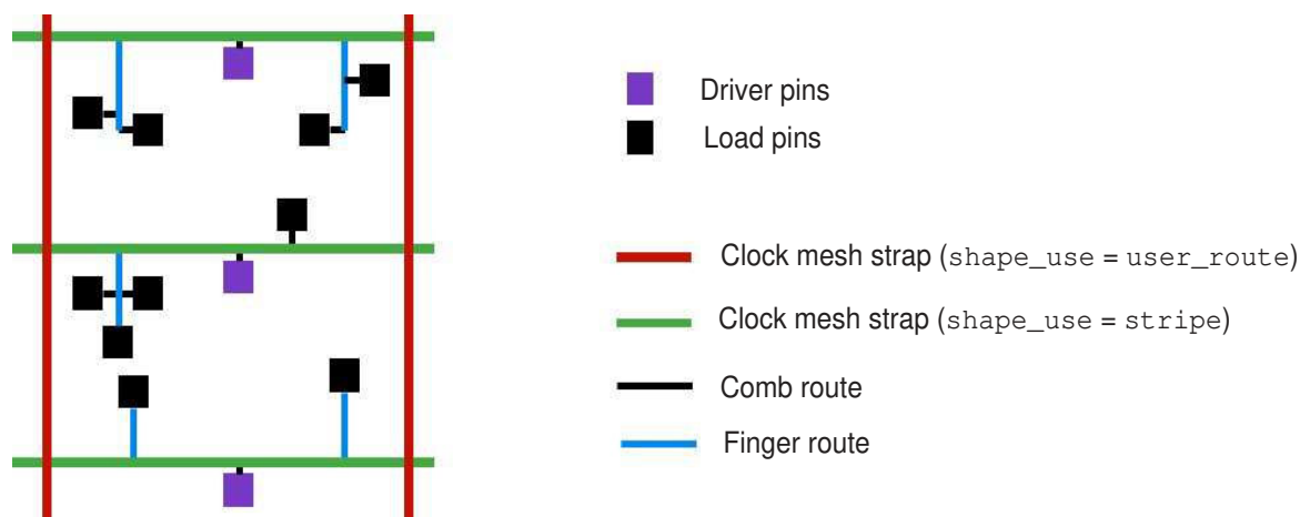
Figure 51 Fishbone Topology
