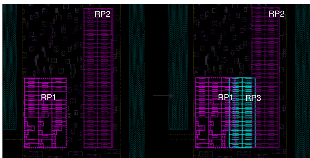
Figure 146 Legalizing the RP3 Relative Placement Group Over Other Groups
