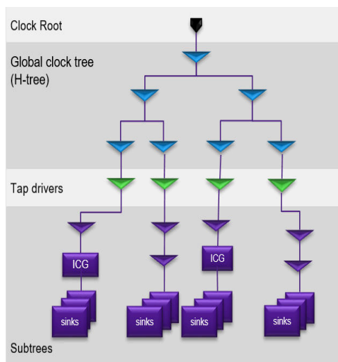
Figure 47 Regular Multisource Clock Tree With an H-Tree-Only Global Clock Structure
