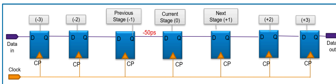
Figure 43 Previous, Current, and Next Path Stages
