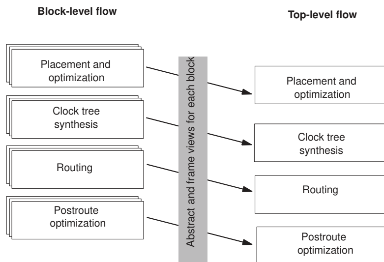
Figure 152 Top and Block Levels Implemented in Parallel
