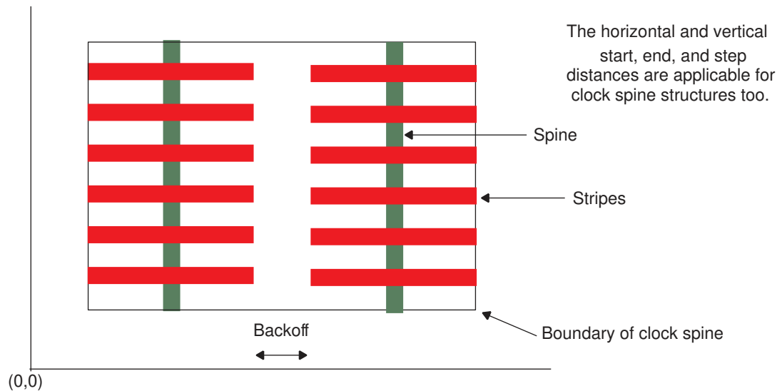
Figure 50 Clock Spine Structure
