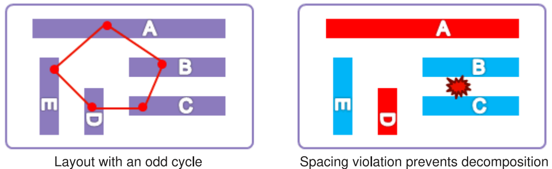
Figure 4 Odd-Cycle Violation
