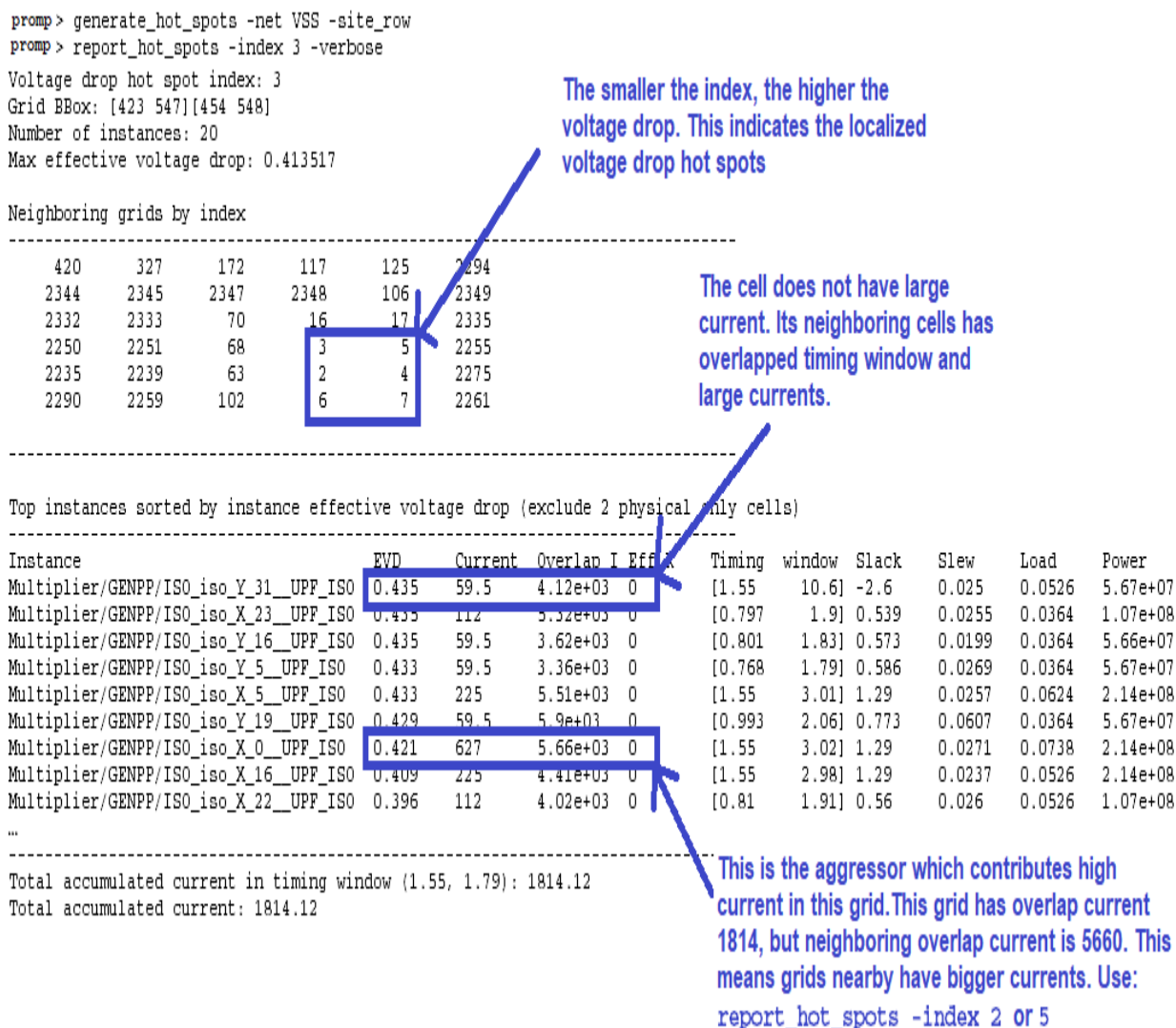
Figure 170 Checking High Voltage Drop Caused by Overlapping Timing Window (I)
