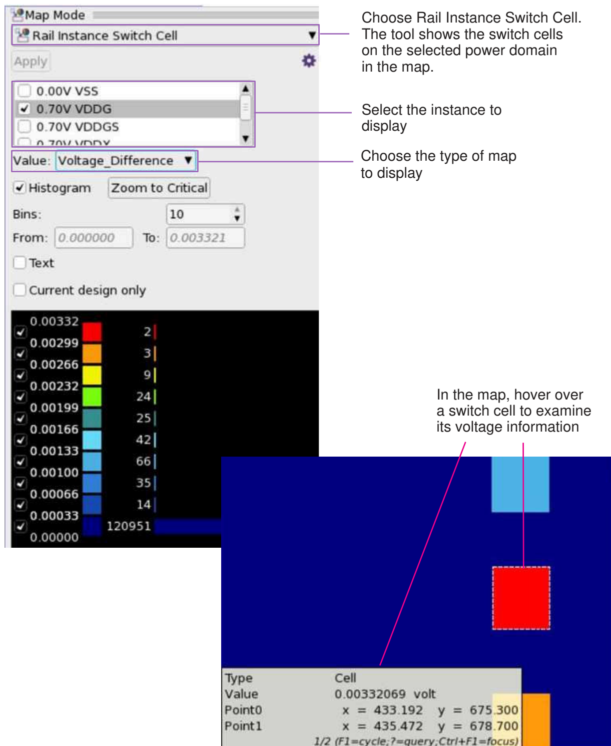
Figure 168 Displaying Maps for Switch Cells
