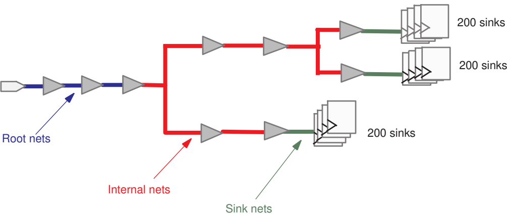
Figure 67 Root, Internal, and Sink Clock Net Types
