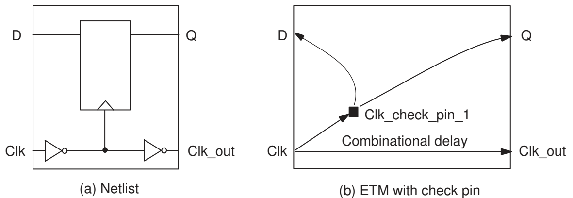
Figure 40 Module With Combinational Clock Path
