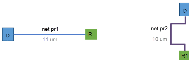
Figure 115 Minimum Wire Length Constraint for pr* Nets
