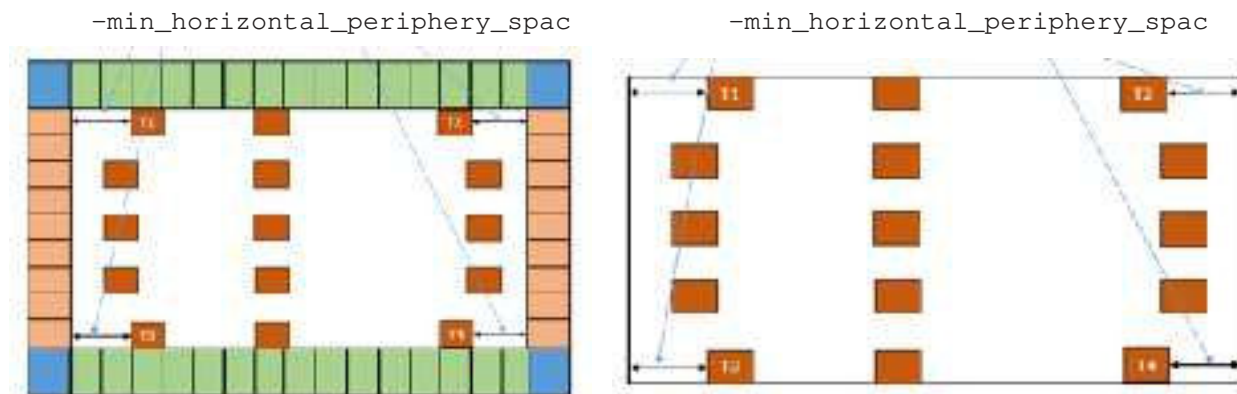
Figure 82 Tap Cell Boundary Row Spacing
