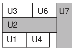
Figure 129 Hierarchical Relative Placement Group With Straddling
