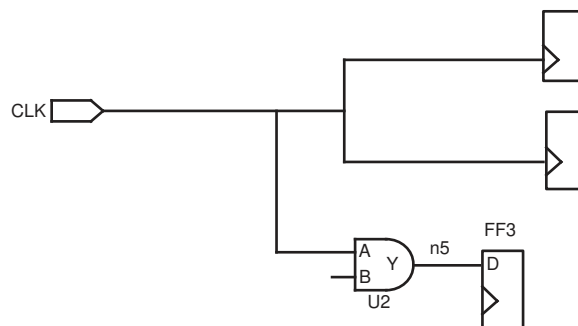
Figure 39 Specifying Exceptions on Pins Beyond the Clock Network
