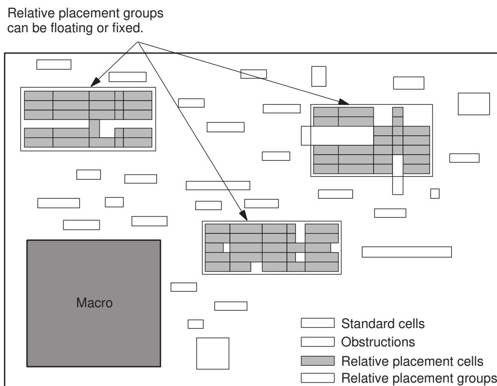
Figure 126 Relative Placement in a Floorplan
