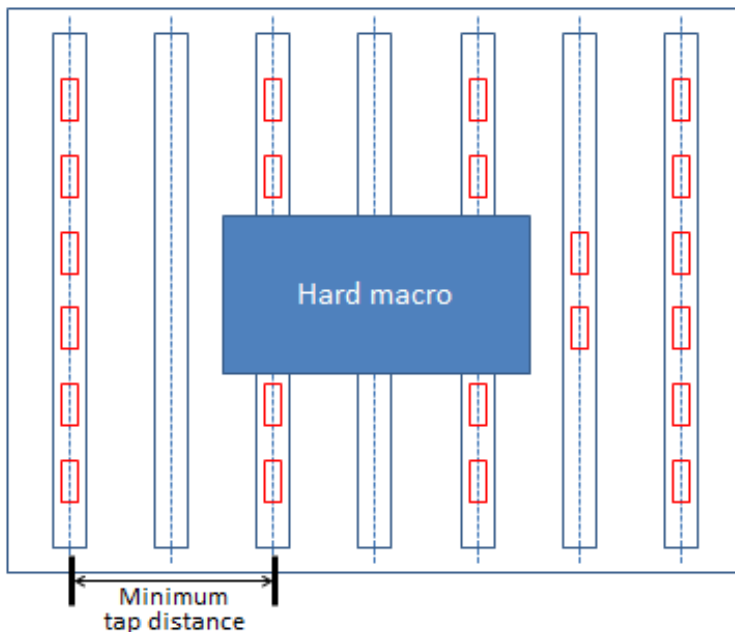
Figure 81 Default Tap Cell Placement
