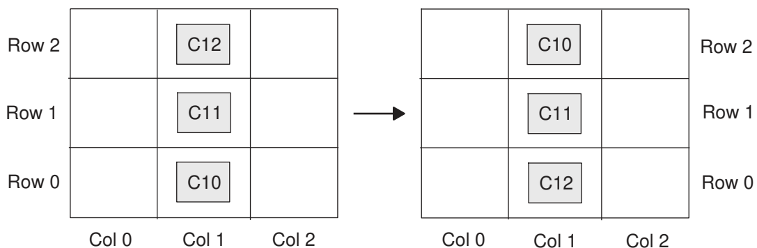
Figure 144 Flipping a Column of a Relative Placement Group
