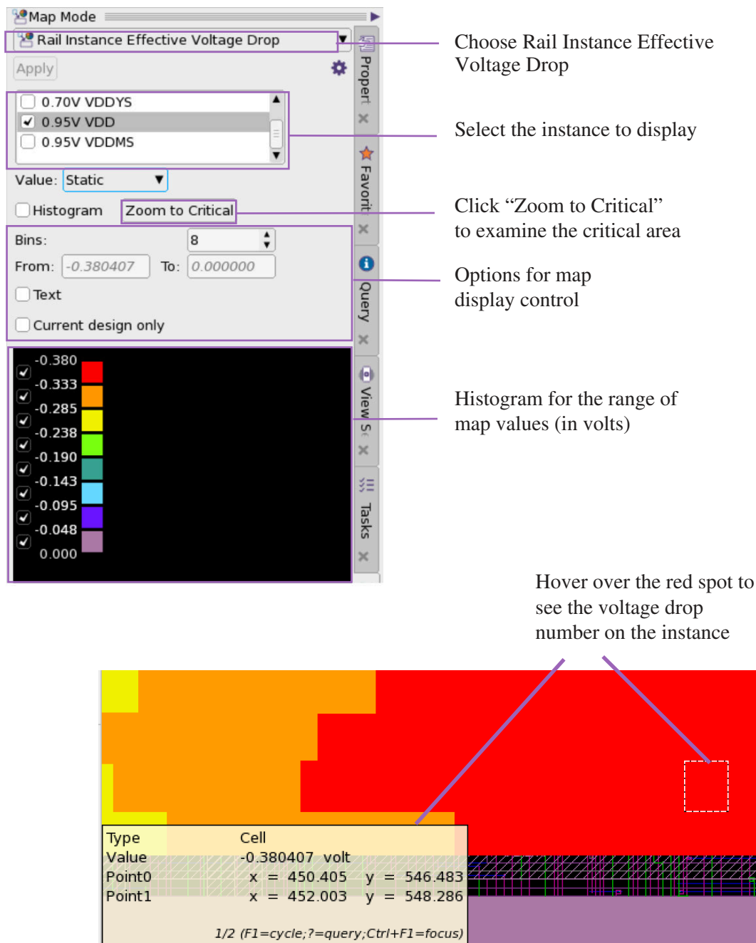
Figure 167 Displaying a Rail Instance Effective Voltage Drop Map
