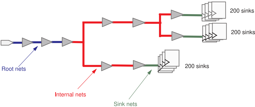
Figure 22 Root, Internal, and Sink Clock Net Types
